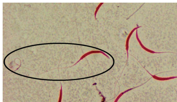
Fig. 7. Midpiece damage
